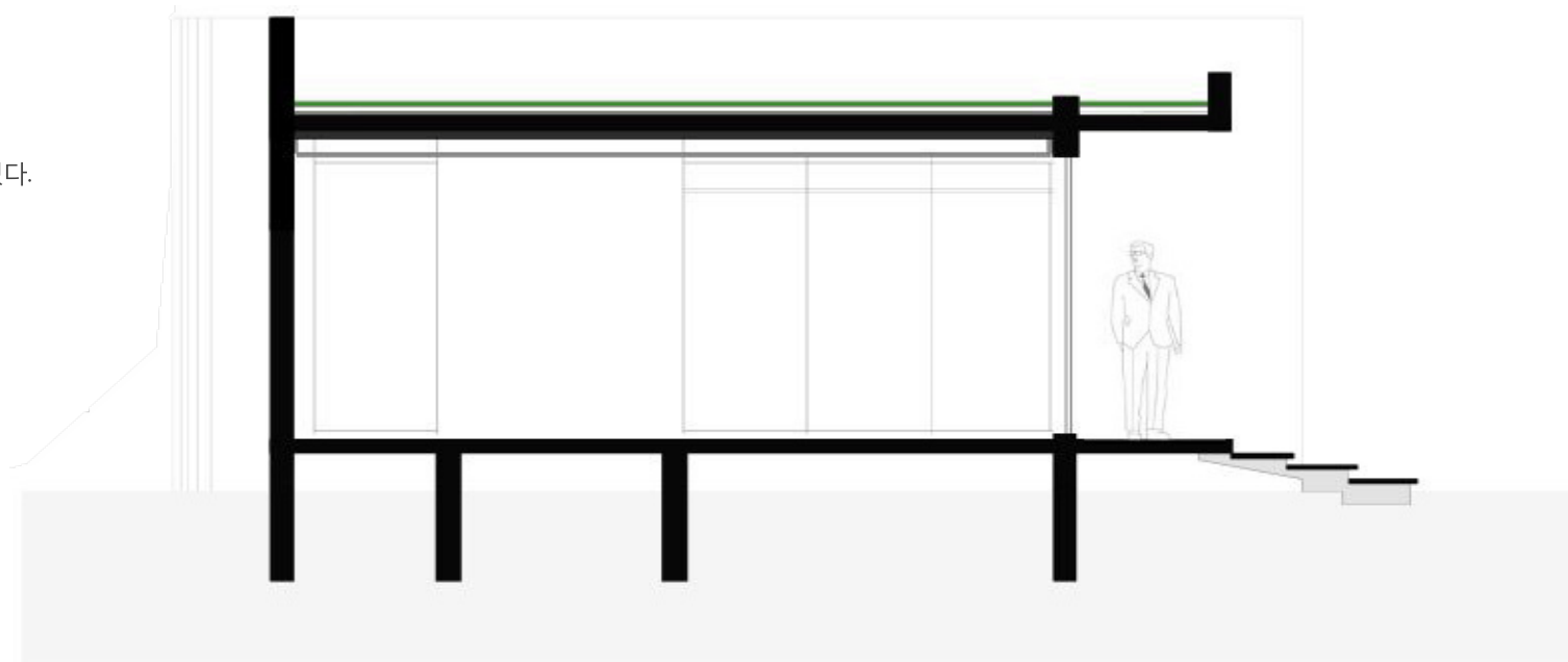
TRANSVERSAL SECTION
